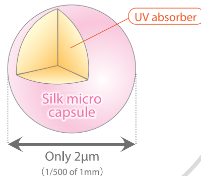
Structure of Silasoma
